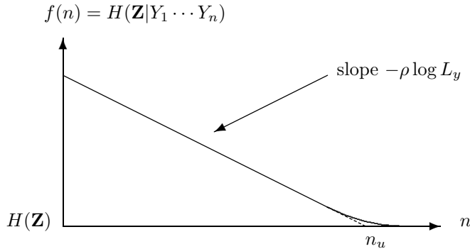
Figure 9.3: The usual form of the key equivocation function for a secret-key cipher.
