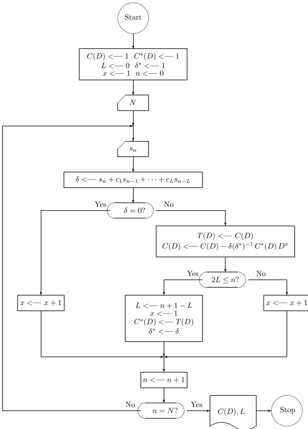
Figure 8.4: LFSR Synthesis Algorithm (Berlekamp-Massey Algorithm) for finding (one of) the shortest LFSR(s) that can generate the sequence s_0, s_1, \dots, s_{N-1} .
